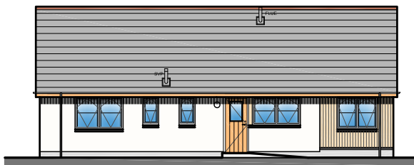
Rear Elevation
