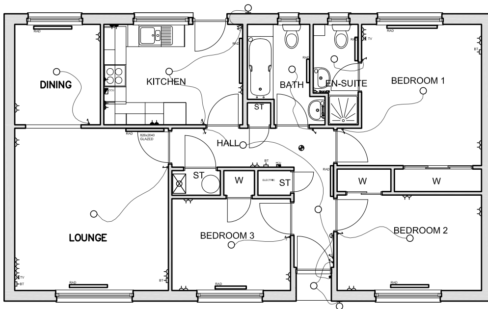
Floor Plan
