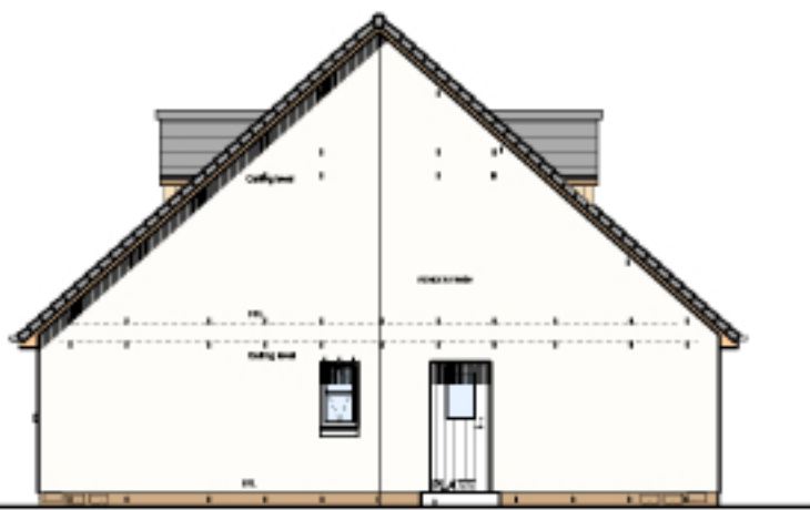
GABLE ELEVATION
